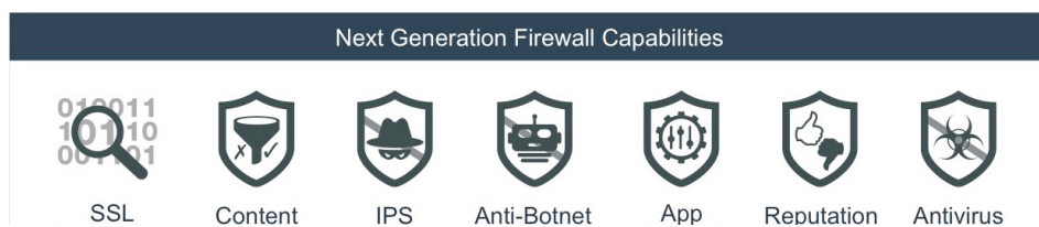
Figure 14: Security requirements.
