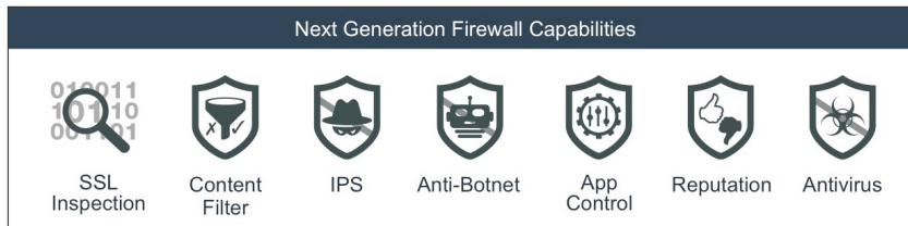
Figure 5: Security requirements.
